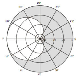
Horizontal Pattern (880MHz)
